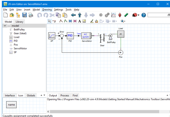
PD controlled servo motor with gearbox and belt.
