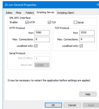
Scripting Interface settings tab.
