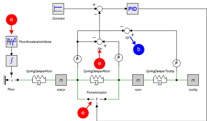
The Dynamic Error Budgeting toolbox shows the total error as a result of injected disturbances.
