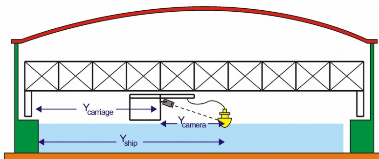
Figure 3: Camera system to measure the ship position.
