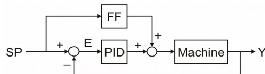
Figure 2: Feed forward control combined with feedback control.
