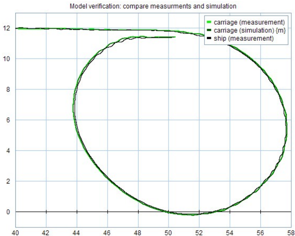
Figure 7: The simulation model shows very accurate predictions of the carriage behavior.
