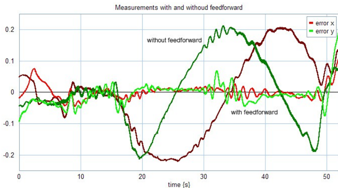
Figure 8: The carriage error during a circle test with and without feed forward control.
