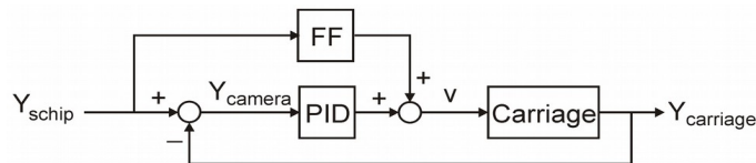
Figure 5: Extension with a feed forward controller that translates the measured ship position into a velocity signal for the motor controllers.
