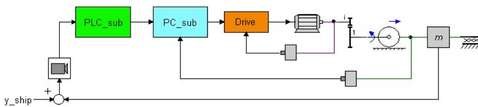
Figure 6: Model of the carriage sub frame created in 20-sim.
