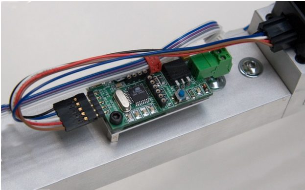
Figure 6: The joint module located on the knee. This board interfaces the encoder, controls the knee-lock magnet, and is connected to the TWI interface using the four colored wires.
