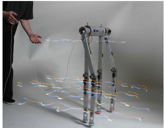
Figure 9: A time-lapse shot of the walking robot.
