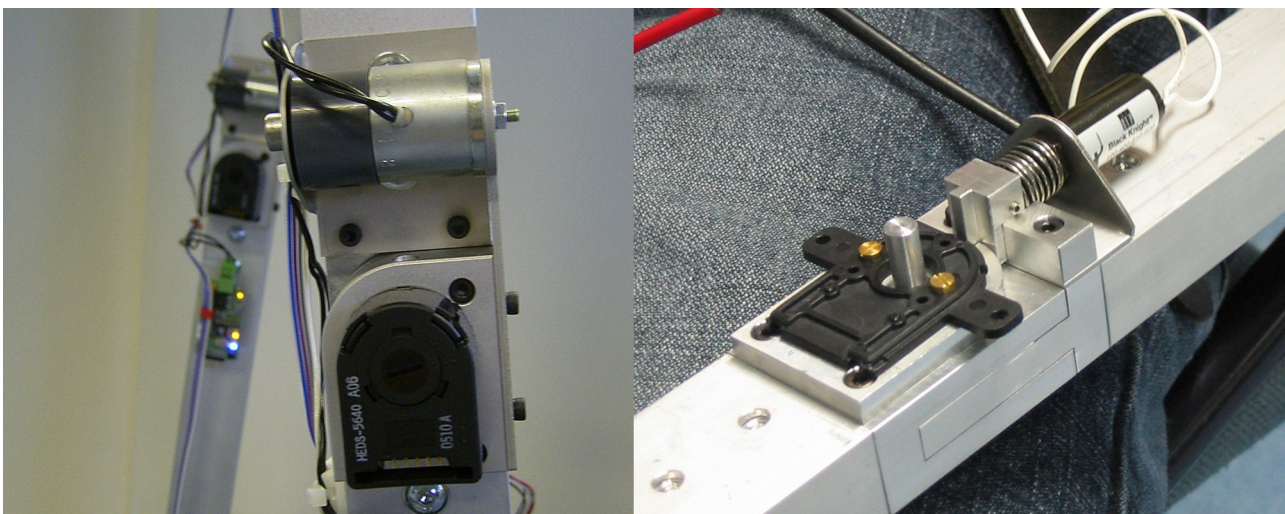
Figure 5: The knee-lock mechanism with locking magnet and the mechanism with retracting pin.
