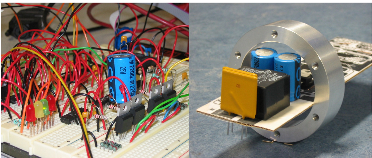
Figure 8: A working breadboard design of the 150-W motor amplifier and a cardboard mock-up of the PCB design.
