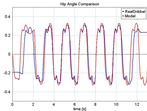
Figure 3: Hip angle during a short, straight walk in both the simulation and real robot.
