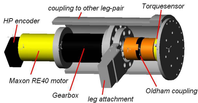
Figure 4: SolidWorks drawing of the drive train.
